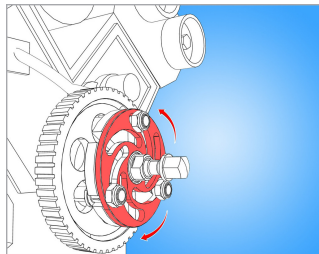
Turn setting plate to shift puller legs, so they tightly grasp to pulley.
