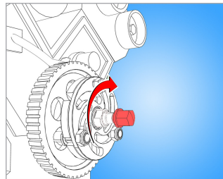
Turn spindle clockwise until pulley comes off.
