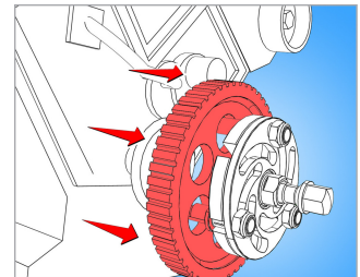
When finished working, remove puller.
