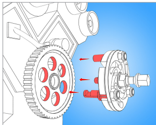
Insert puller legs into openings of pulley.
